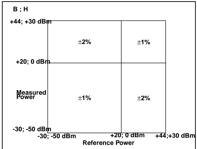
Figure 19 Relative Mode Power Measurement Linearity with Agilent EPM power meter at 25°C ±10°C (typical)
